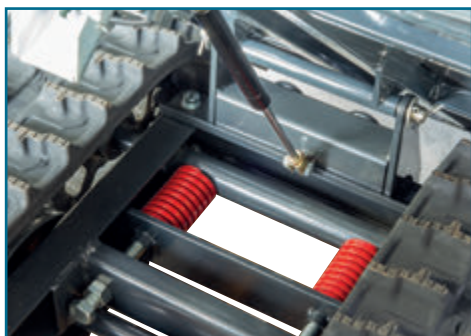
Tendingoli - dampers
